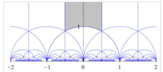
The action of the modular group on the upper half plane. The region in grey is the standard fundamental domain.
