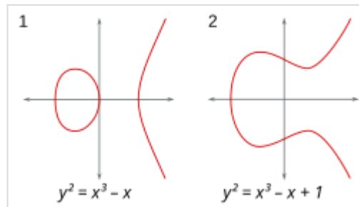
Two examples of elliptic curves , that is, curves of genus 1 having at least one rational point
