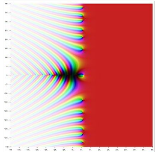
Riemann zeta function \zeta(s) in the complex plane. The color of a point s gives the value of \zeta(s) : dark colors denote values close to zero and hue gives the value's argument.
